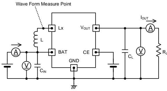
< Circuit No.① >
