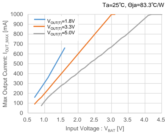
XC9147, f_{OSC}=1.2MHz
