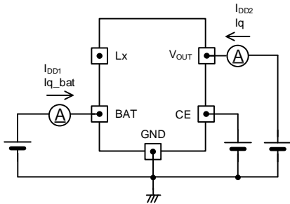
< Circuit No.③ >
