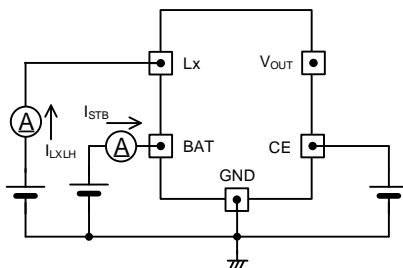
< Circuit No.⑦ >
